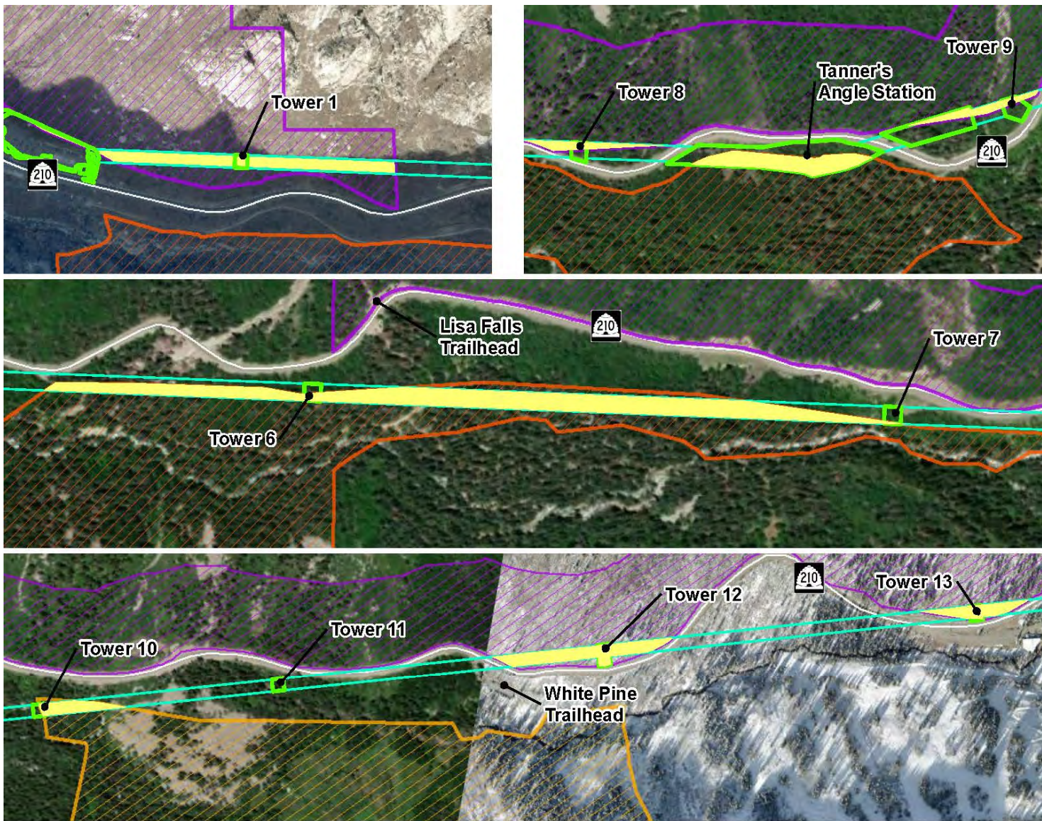
Figure 6. Gondola Alternative A
