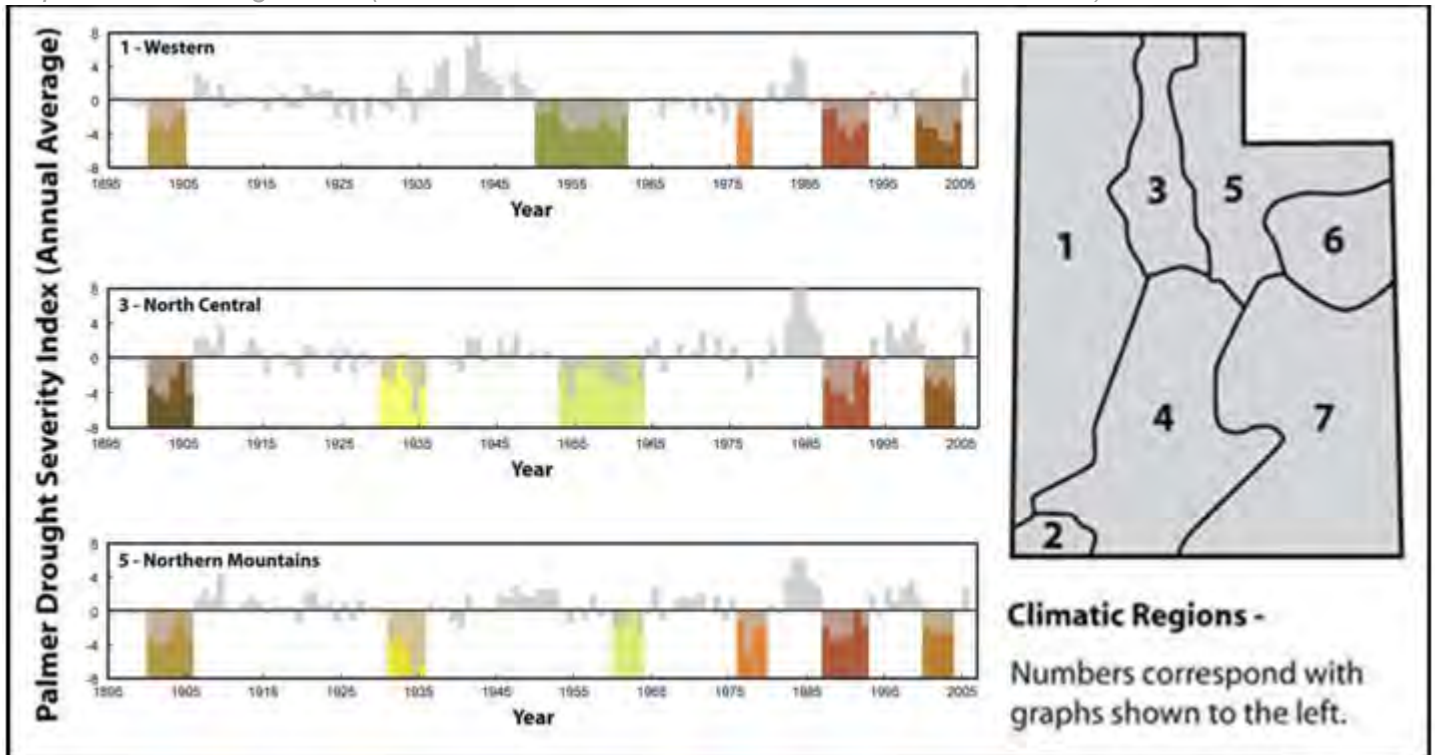
Map: Annual Average PDSI (Modified from Utah Division of Water Resources 2007a)
