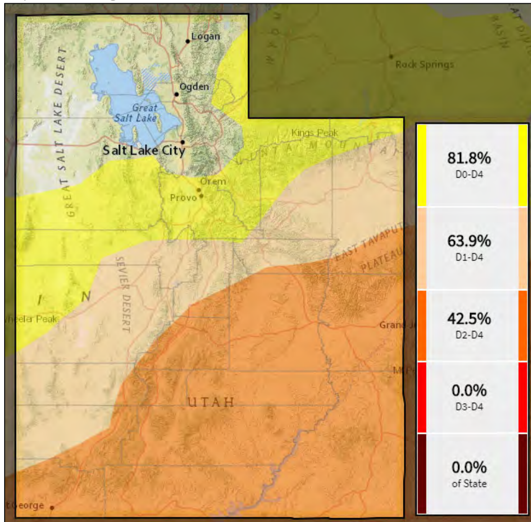
Map: Utah Drought Extent, November, 2019
