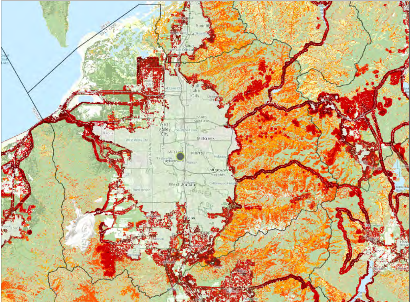
Map: Salt Lake County Wildfire Aggregate Value Impacts
