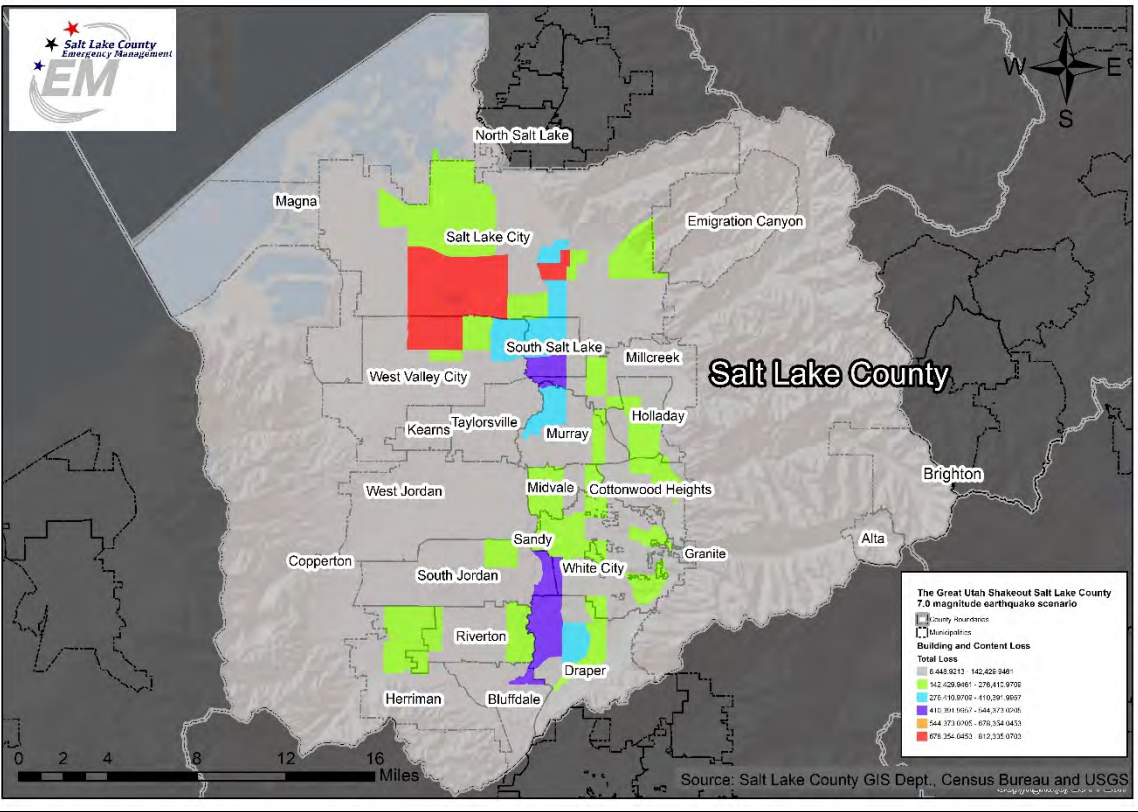
Map: Salt Lake County Shake Map for M7 Event: Building and Content Loss (Great Shakeout)
