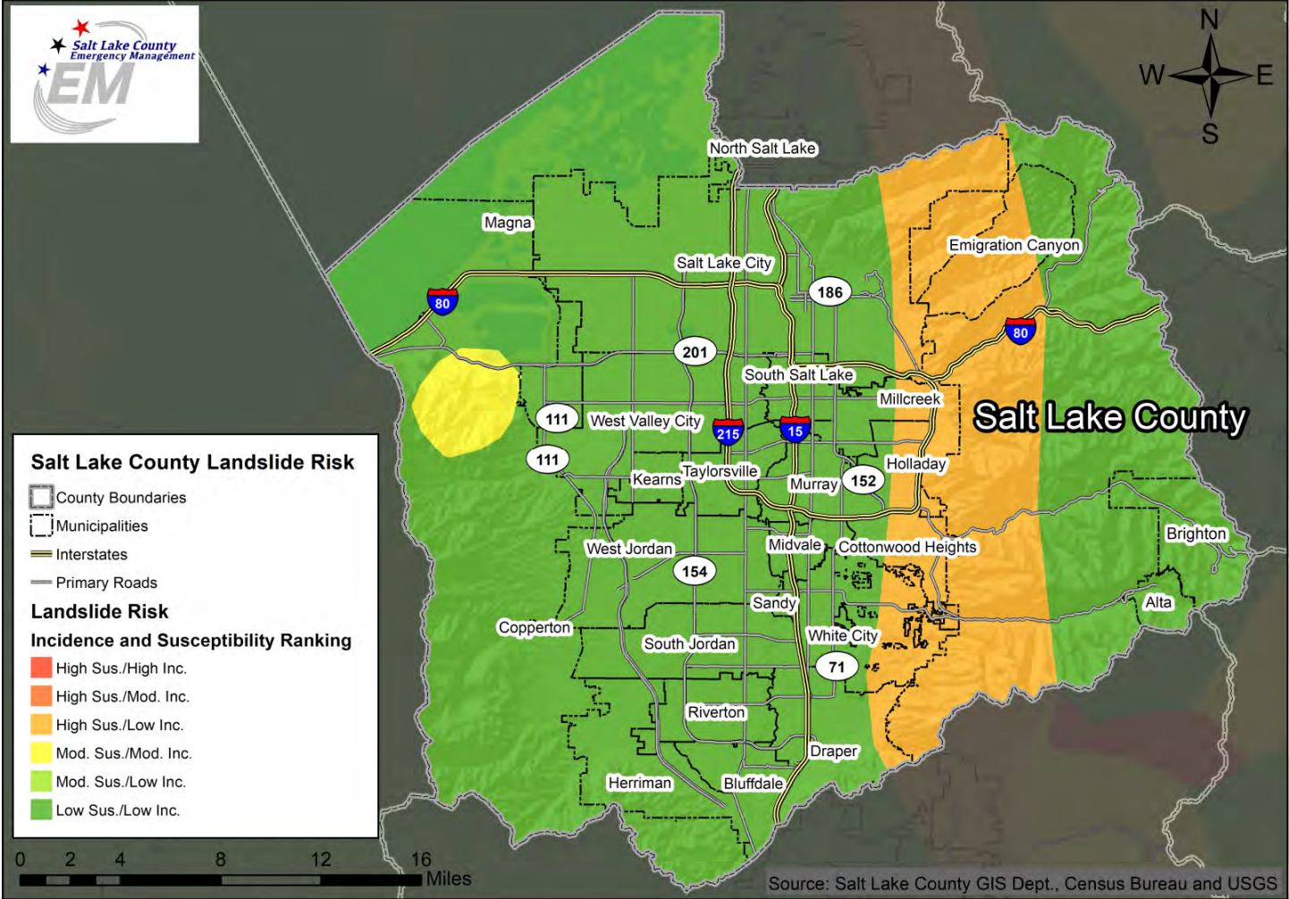
Map: Salt Lake County Landslide Risk
